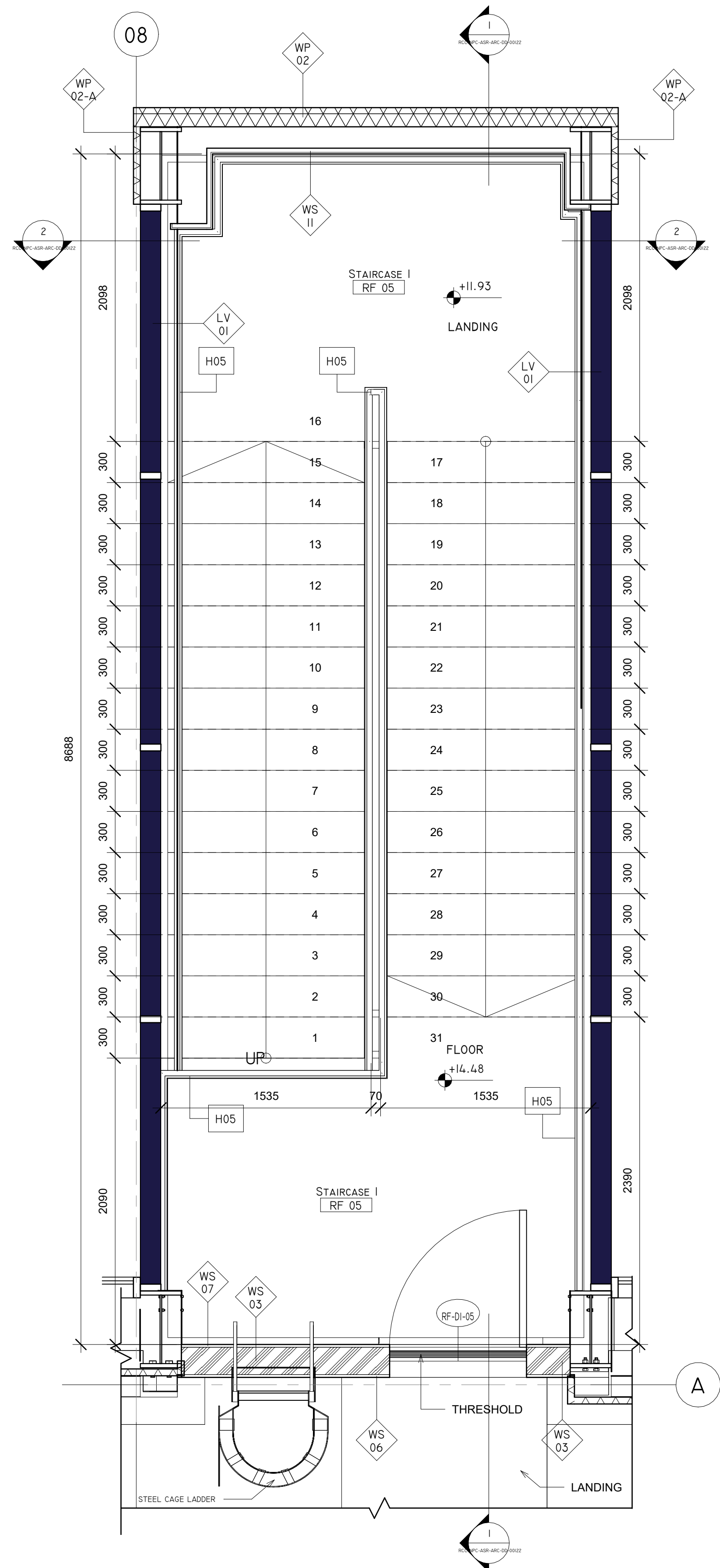
04 ROOF FLOOR PLAN (STAIRCASE -I) 1 : 25
