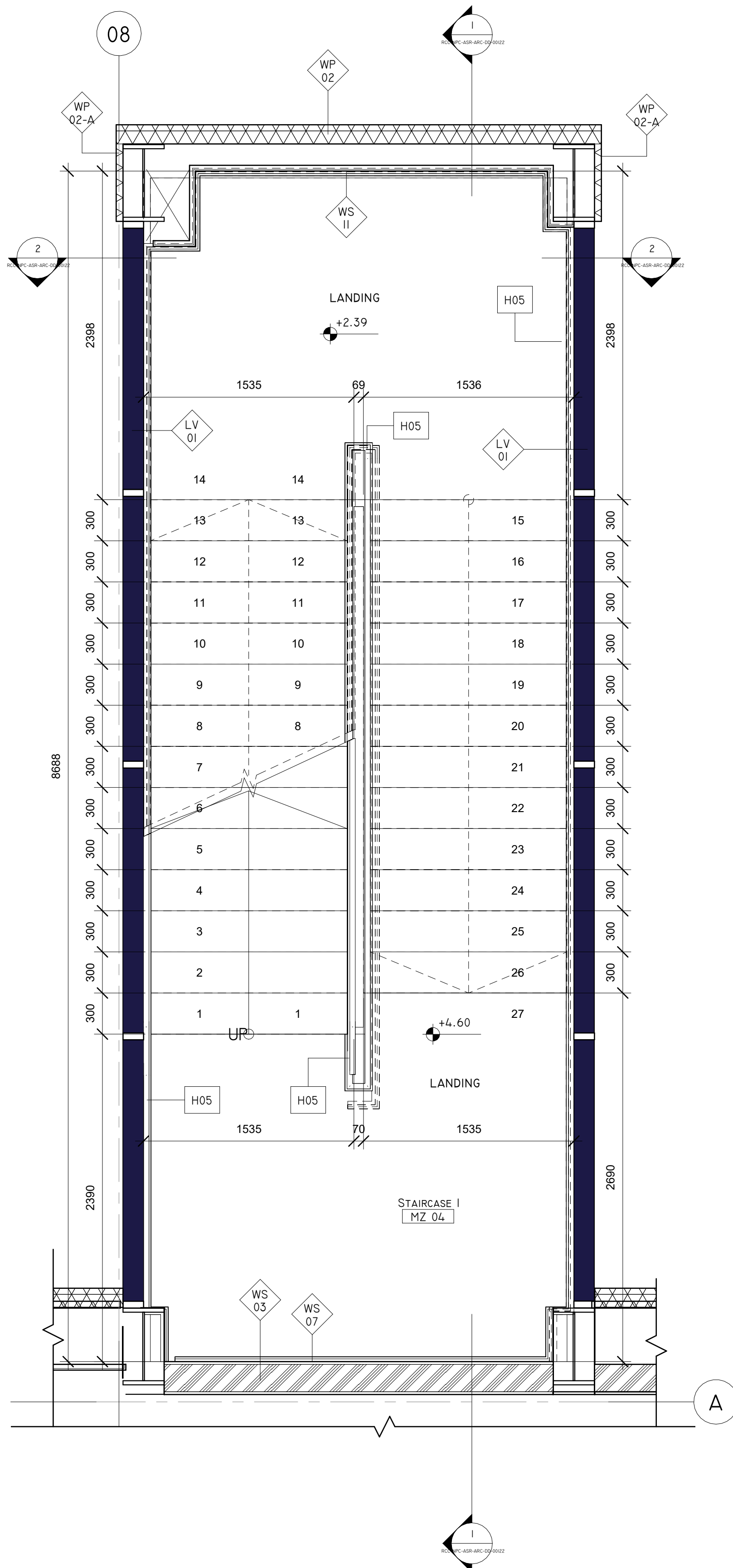
02 MEZZANINE FLOOR PLAN (STAIRCASE -I) 1 : 25
