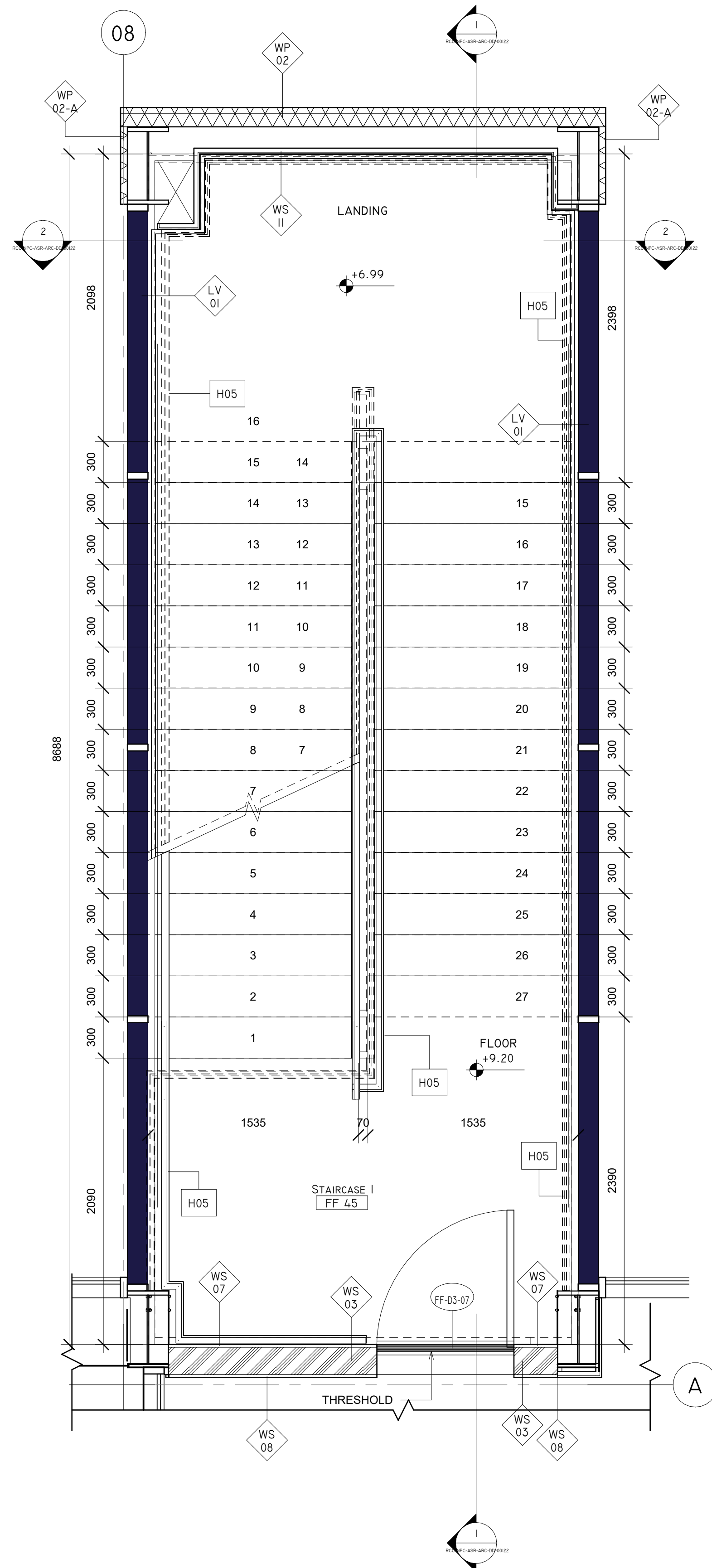
03 FIRST FLOOR PLAN (STAIRCASE -I) 1 : 25
