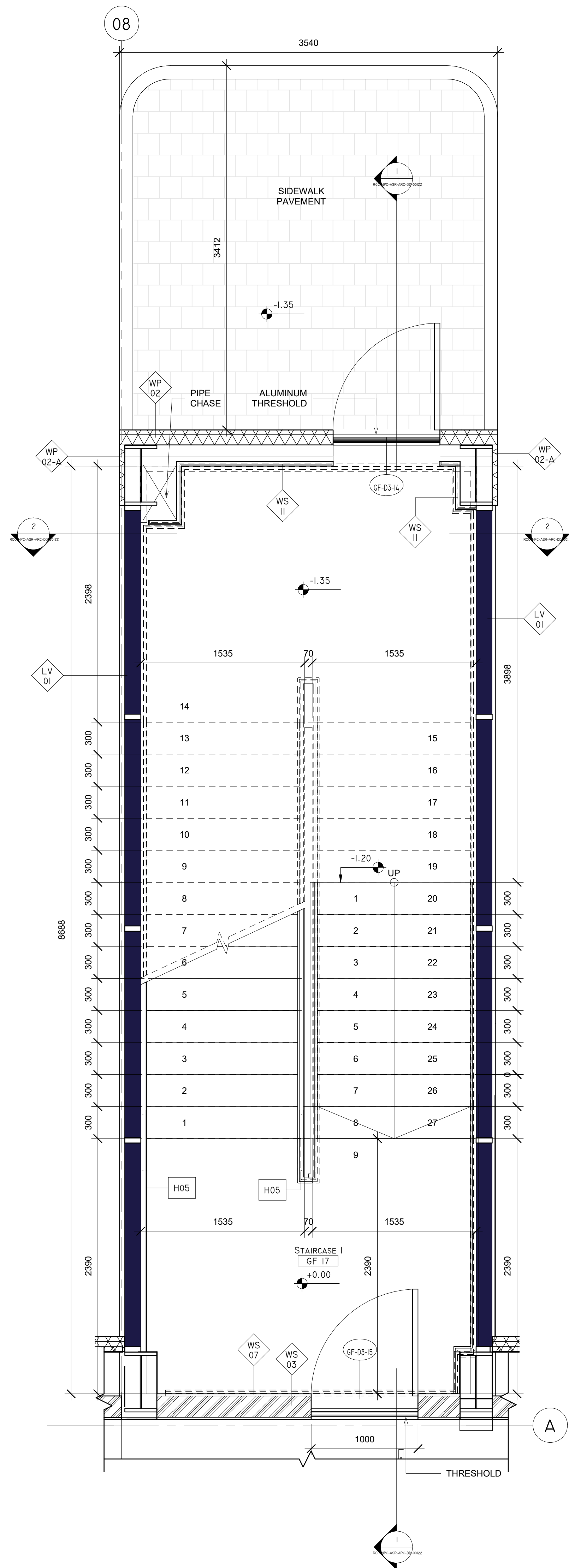
01 GROUND FLOOR PLAN (STAIRCASE -I) 1 : 25
